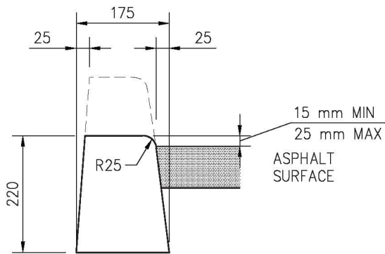
150mm SEPARATE CURB
