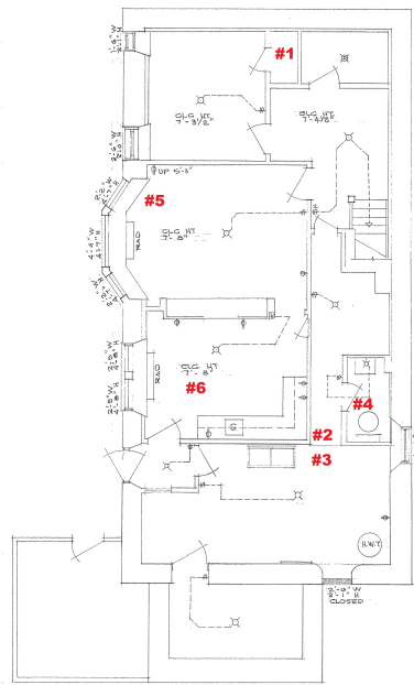
LOWER FLOOR 1/4" = 1'-0"
