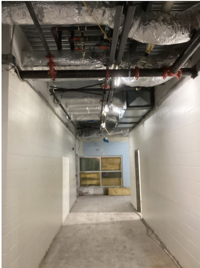
Corridor adjacent to lobby: Sprinkler, HVAC, and electrical work completed; painting finished; ready for acoustic tile ceiling installation
