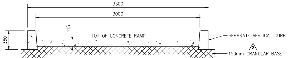
SECTION B-B SCALE 1:50
