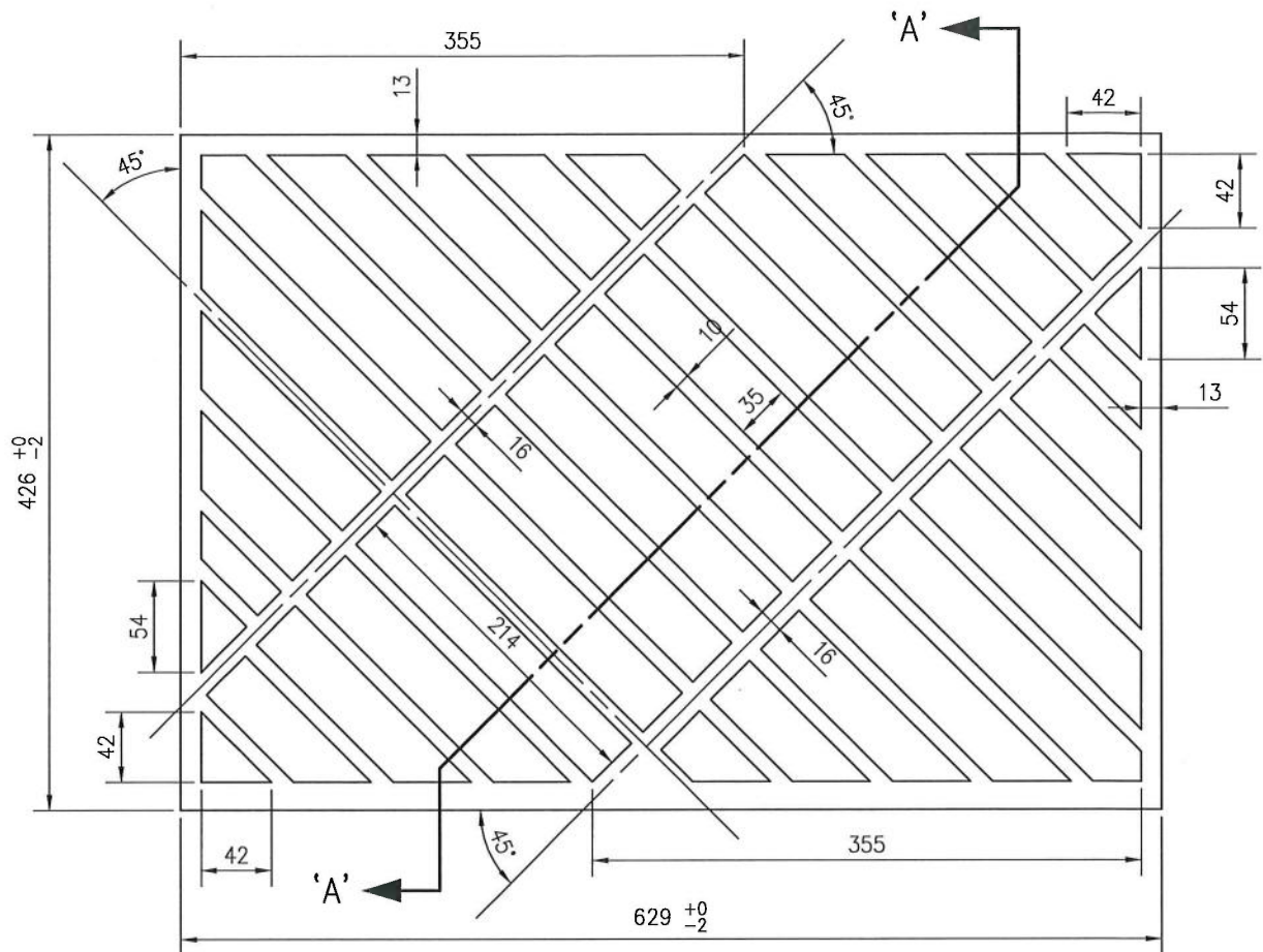
PLAN VIEW
