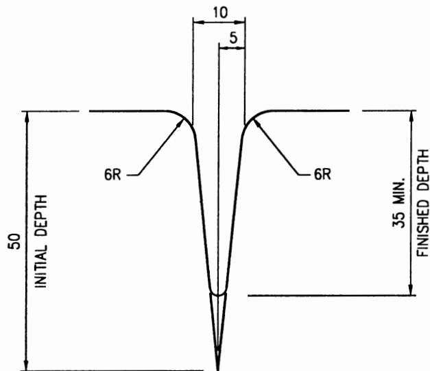
LONGITUDINAL CONTROL JOINT
