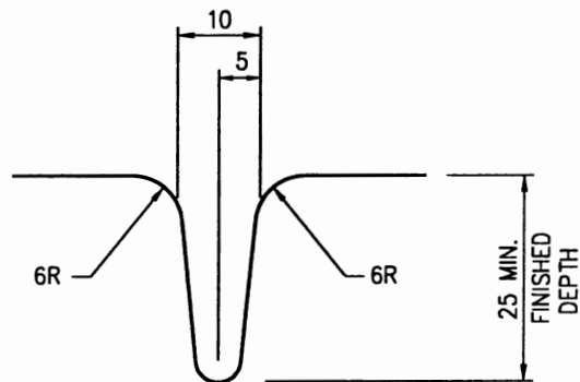
TRANSVERSE CONTROL JOINT
