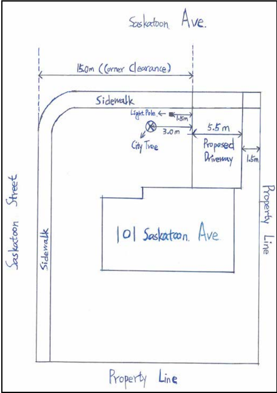
Hand Sketch
