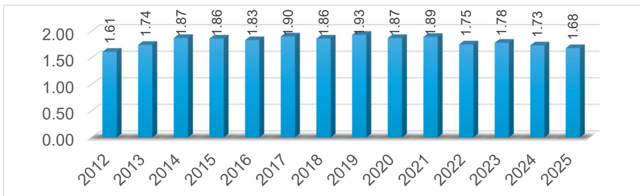
Figure 3.4 - Ratio of Treated Water Maximum Day Pumpage to Average Dry Pumpage
