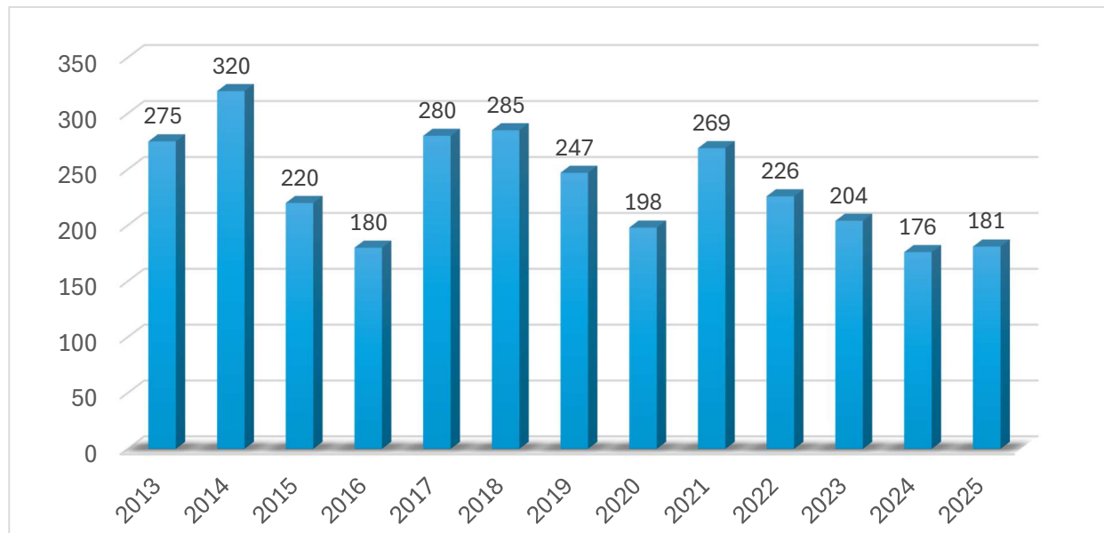
Figure 5.3 - Quantity of Water Main Breaks per Year
