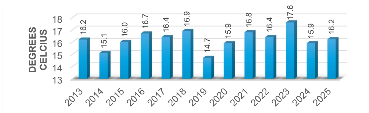
Figure 3.3 - Saskatoon Seasonal Mean Temperature, Deg. Celsius (May to August) Source: Environment Canada
