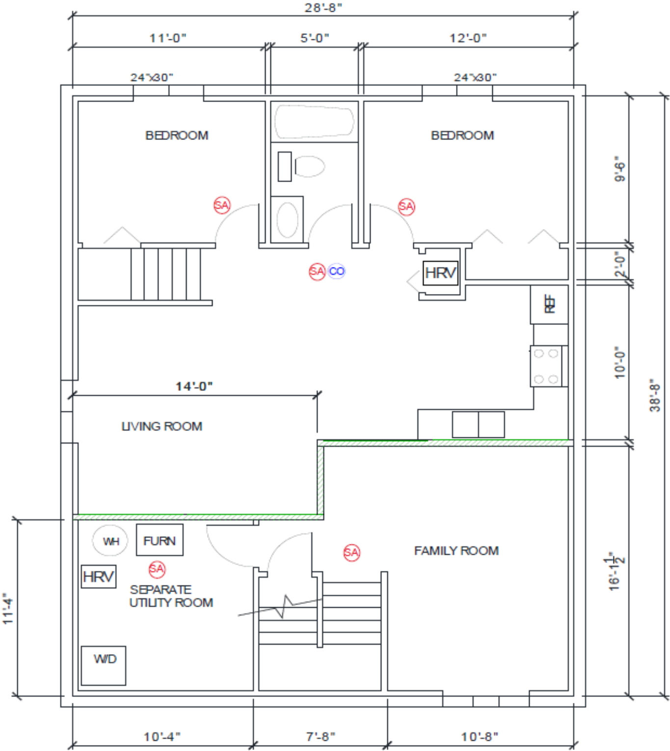
Plan 3 – Separate entrance, separate utility room
