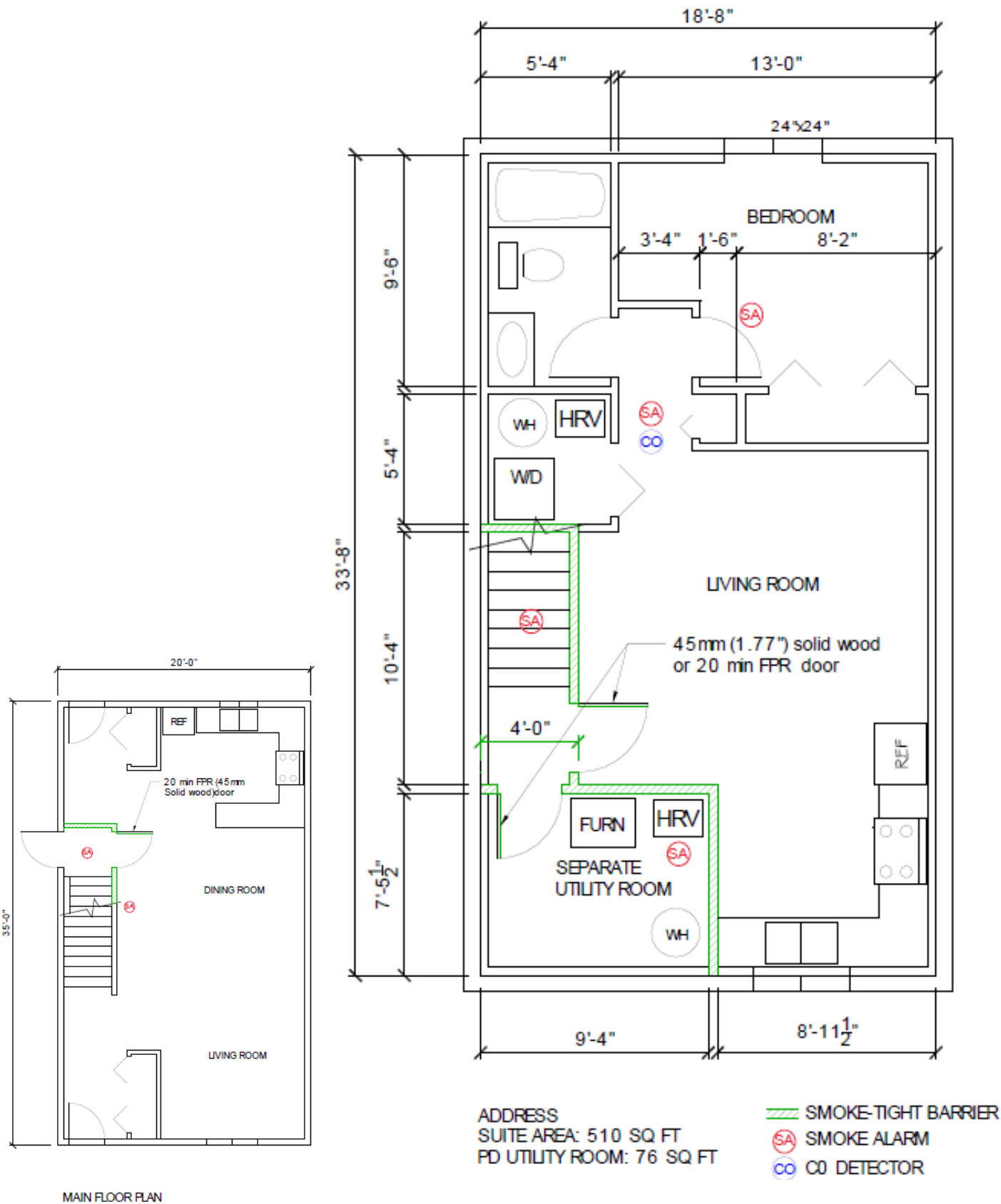
Plan 1 – Separate utility rooms, common stairwell
