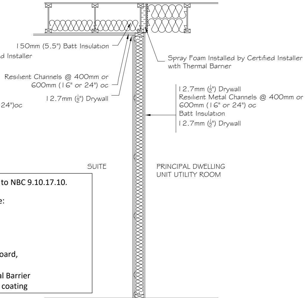
WALL SECTION 4 SMOKE TIGHT BARRIER (SPRAY FOAM) EXTENDING TO UNDERSIDE OF SUBFLOOR JOISTS PARALLEL TO WALL
